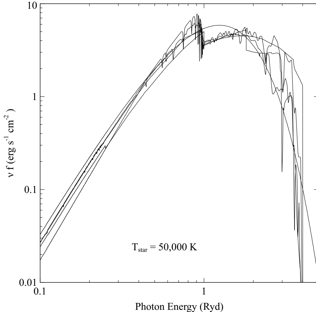
Figure 6.4: This figure shows the emergent radiation field predicted by five 50,000 K stars included with the code. The smoothest is the blackbody, and the Kurucz (1991) and Rauch (1997) atmospheres show the most structure. stars
