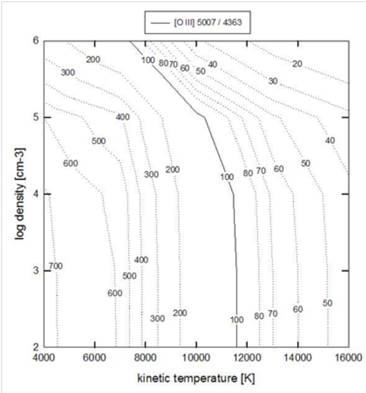
Figure 15.3: The [O III] line ratio as a function of density and temperature.
