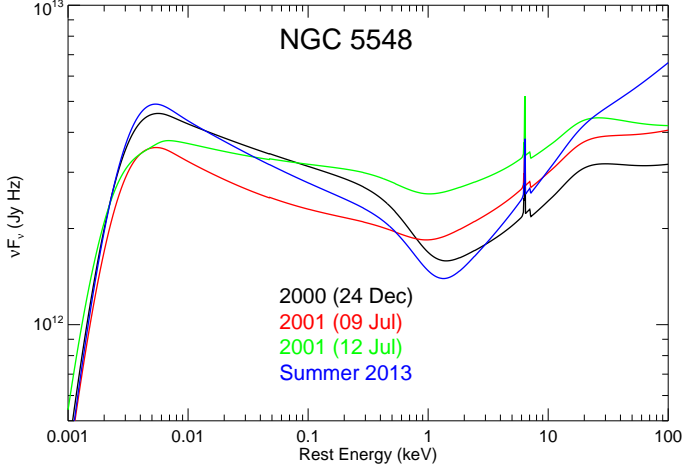
Fig. 11. The broadband continuum SED models for the unobscured (2000, 2001) and obscured (2013) epochs of NGC 5548, obtained in Sect. 6.
