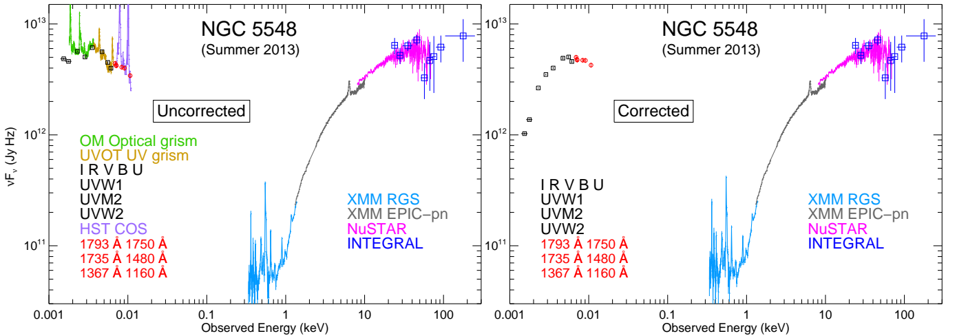
Fig. 6. Average multi-wavelength data of NGC 5548 from our summer 2013 campaign. The data are displayed before ( left panel ) and after ( right panel ) corrections for Galactic reddening (Sect 4.1), host galaxy stellar emission (Sect 4.2), emission lines from the BLR and NLR (Sect 4.3), blended Fe II emission (Sect. 4.4), Balmer continuum (Sect. 4.5) and Galactic interstellar X-ray absorption (Sect 4.6). The spectra have been binned for clarity of presentation. The displayed X-ray data include the effects of heavy absorption by the obscurer and the warm absorber. The shape of the NIR/optical/UV data after the corrections ( right panel ) is remarkable and exhibits a thermal disk spectrum.
