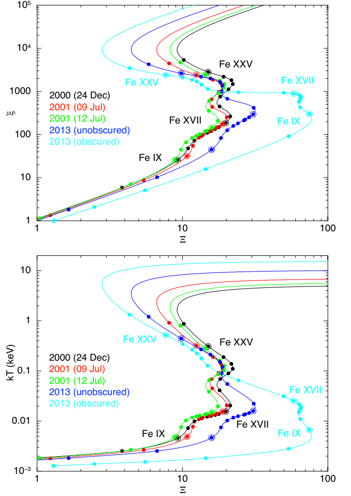
Fig. 13. Thermal stability curves for photoionised gas in NGC 5548, showing \xi plotted versus \Xi ( top panel ) and temperature kT plotted versus \Xi ( bottom panel ). They have been calculated for SEDs (displayed in Figs. 11 and 12) derived from our broadband modelling of the continuum as described in Sect. 6. The circles on the stability curves indicate the positions at which ionic column densities of Fe peak on the (\Xi, \xi) and (\Xi, T) phase space. To guide the eye, the location of Fe IX, Fe XVII, Fe XXV have been indicated with open circles around filled circles.
