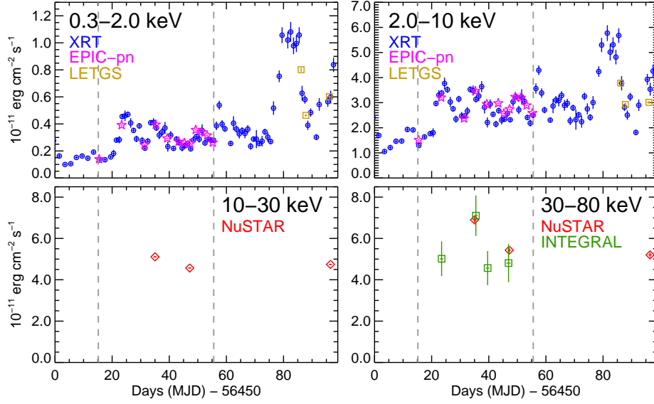
Fig. 2. X-ray lightcurves of NGC 5548 from our summer 2013 campaign. The lightcurves show the observed flux and are displayed between 7 June and 14 Sep 2013. The XRT data are shown as blue circles, EPIC-pn as magenta stars, LETGS as dark yellow squares, NuSTAR as red diamonds and INTEGRAL data as green squares. The vertical dashed lines indicate the interval between XMM-Newton Obs. 1 and 12.
