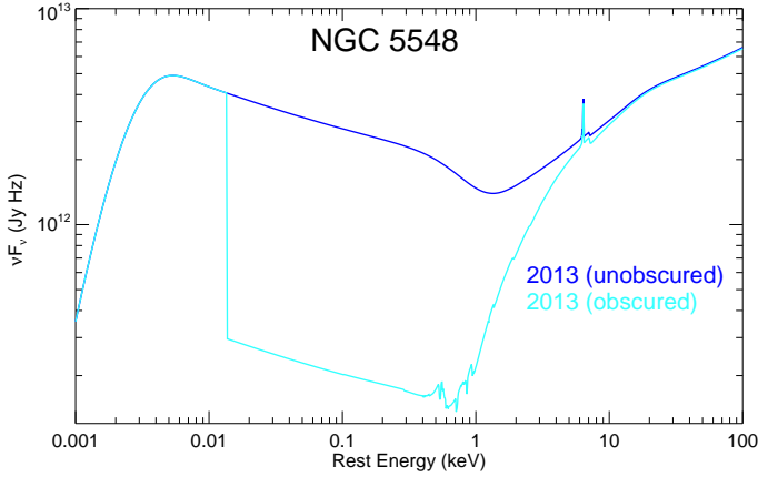
Fig. 12. The SED model for the 2013 epoch, displayed before ( dark blue ) and after ( light blue ) absorption of the continuum by the obscurer. The ionising luminosity L_{1-1000 \text{ Ryd}} is 11.7 \times 10^{43} erg s ^{-1} before obscuration and 3.5 \times 10^{43} erg s ^{-1} after obscuration.
