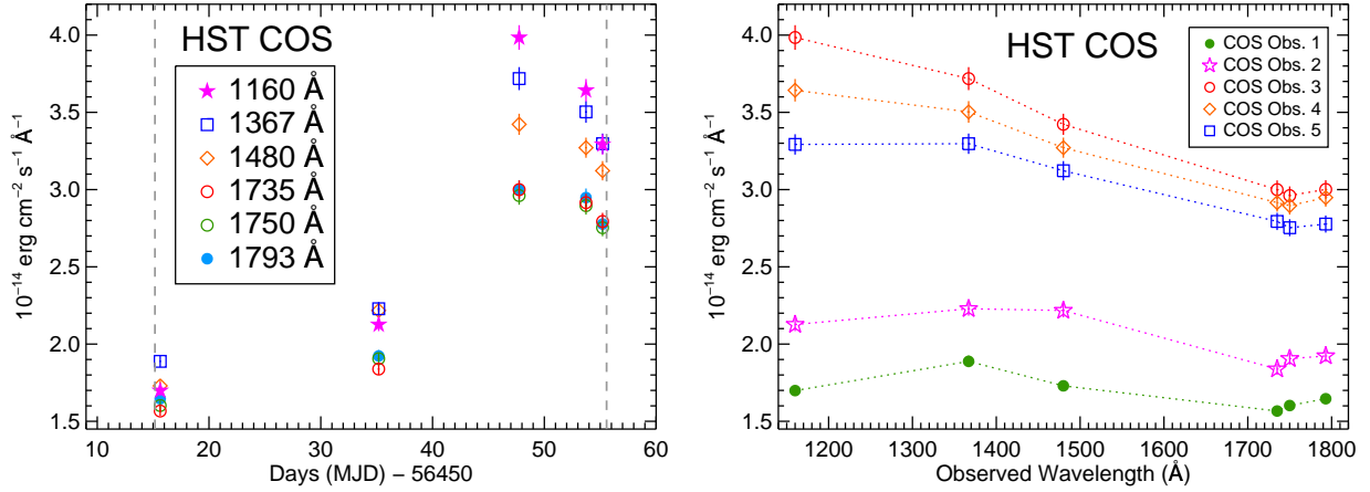
Fig. 4. HST COS fluxes of NGC 5548 at different UV wavelengths from summer 2013 observations. The lightcurves ( left panel ) and spectra ( right panel ) show the observed energy flux obtained from narrow energy bands which are free of spectral features. The displayed range of the lightcurves is between 16 June and 6 August 2013, with the vertical dashed lines indicating the interval between XMM-Newton Obs. 1 and 12.
