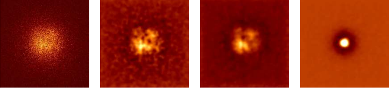
Figure 7. Artificial photon images for the 10^{15} h^{-1} M_{\odot} isolated galaxy cluster obtained with the X-MAS software package. In all the panels, photons have been selected in the energy band \Delta E = [0.3, 1.5] keV, maps were binned in 4pix/bin, and the physical scale of the maps is \sim 670 kpc. The cluster emissivity map before applying any smoothing is illustrated in the first panel, while all the other panels have been obtained by unsharp masking previously smoothed images, as explained in the text. The second and the third panels show qualitatively very similar features. They are for the run with AGN feedback and differ only in the exposure time. Finally, the fourth panel shows how the same cluster appears when the bubble heating is absent.
