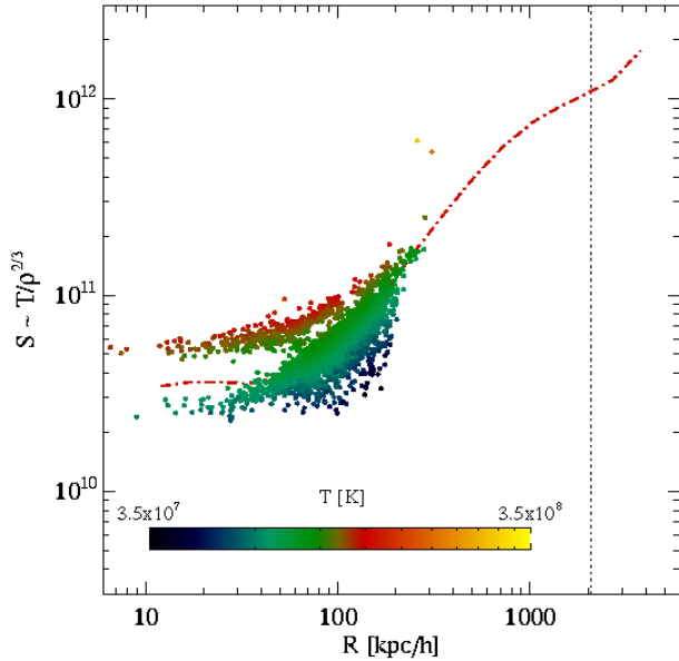
Figure 5. Mean radial entropy profile of the 10^{15} h^{-1} M_{\odot} isolated halo. The result for the simulation with AGN feedback is given by the red dot-dashed line. The dots show the positions of the bubble particles, and they are colour-coded according to their temperature.
