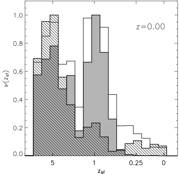
Figure 11. Distribution of formation redshifts of the stars belonging to the cD galaxy of the S1 galaxy cluster at z = 0 . The white histogram corresponds to the case with cooling and star formation only; here it can be seen that stars continue to be formed until z = 0 . The grey coloured histogram shows how the stellar formation times change when our “Magorrian model” of bubble heating is switched on, which essentially suppresses any central star formation for z < 0.25 completely. Finally, the result for the “BHAR model” of AGN feedback is illustrated with the hatched histogram, which shows a considerable suppression of central star formation at intermediate redshifts, 0.3 < z < 2.0 .
