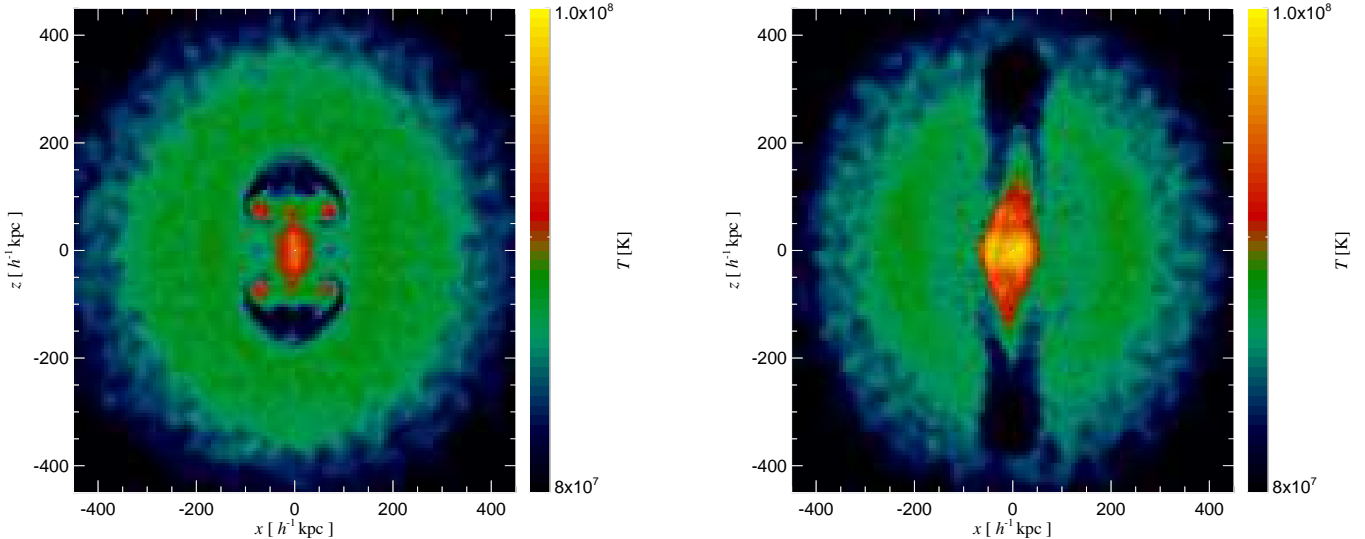
Figure 2. Time evolution of the isolated 10^{15} h^{-1} M_{\odot} galaxy cluster with a jet-like AGN heating. The models are the same as in Figure 1, only the bubbles have two times bigger radii, namely 60 h^{-1} kpc. It can be noticed how the morphology in the central cluster region changes due to bubble-induced motions, from \sim 1.8 Gyr (left panel) to \sim 3.3 Gyr, when a well-defined bipolar outflow is clearly visible (right panel).
