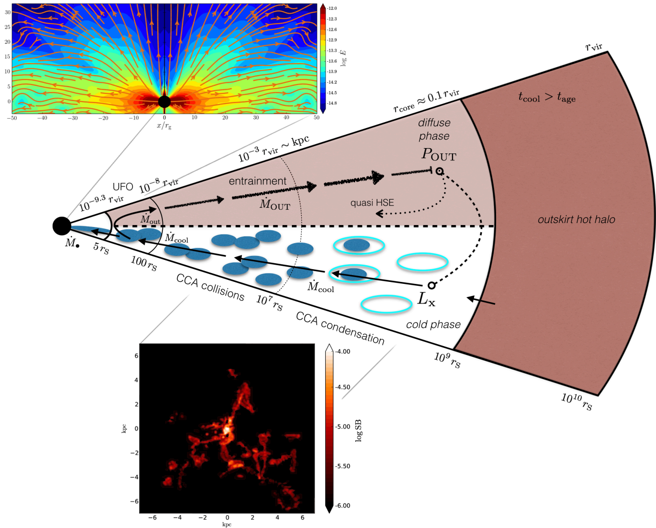
Figure 1. Middle – Diagram of the multiphase accretion inflow and outflow covering the entire range of scales, from the inner SMBH horizon to the virial radius of the galaxy, group, or cluster. The self-regulated AGN feedback loop works as follows. The turbulent gaseous halo condenses in localized, large-scale high density peaks (cyan), leading to the drop out of cold clouds and warm filaments (blue). The clouds rain down and recurrently collide in chaotic and inelastic way (CCA), canceling angular momentum and flowing toward the SMBH. The mass inflow rate originates from the quenched X-ray cooling rate within the core region. Within \sim 100 r_S , the gravitational accretion process releases ultrafast outflows (UFOs), while only a small gas fraction is sunk through the horizon (this is balanced by a net inflow from the outskirts). The outflows slow down at larger radii, entraining the gas of the background profile. The energy is thermalized in the core, balancing the X-ray luminosity. The CCA rain is thus stopped, and so are the outflows, allowing the global halo to restore the quasi HSE profile. As cooling resumes without a source of heating, another cycle of CCA rain and collisions, mass ejection and entrainment, and restoration is triggered, consistently with X-ray data. The system conserves total energy and mass in a gentle recycling multiphase flow. Top – GR-RMHD simulation of the micro flow (§2.2), showing the magnitude and streamlines of the total energy flux (from Sądowski et al. 2016; code units) which is dominated by the kinetic component with \epsilon_* \simeq 0.03 (see SG17 for more details on the mechanical efficiency). Bottom – Multiphase hydro simulation of the macro flow tracking the CCA evolution (from Gaspari et al. 2017; §2.1). The map shows the surface brightness ( \text{erg s}^{-1} \text{cm}^{-2} \text{sr}^{-1} ) of the filamentary warm phase condensed out of the turbulent hot halo and chaotically colliding.
