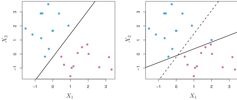
FIGURE 9.5. Left: Two classes of observations are shown in blue and purple, along with the maximal margin hyperplane. Right: An additional blue observation has been added, leading to a dramatic shift in the maximal margin hyperplane shown as a solid line. The dashed line indicates the maximal margin hyperplane that was obtained in the absence of this additional point.
