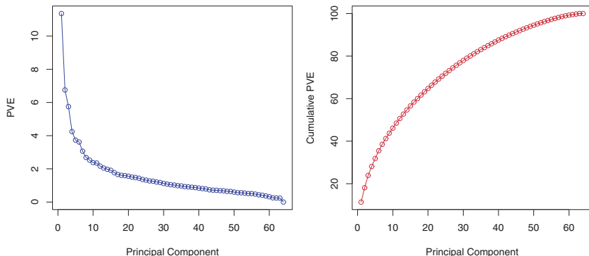
FIGURE 10.16. The PVE of the principal components of the NCI60 cancer cell line microarray data set. Left: the PVE of each principal component is shown. Right: the cumulative PVE of the principal components is shown. Together, all principal components explain 100% of the variance.
